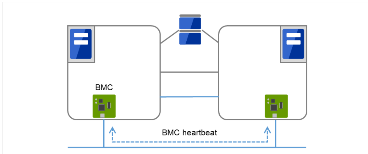
Fig. 3.6: BMC heartbeat
