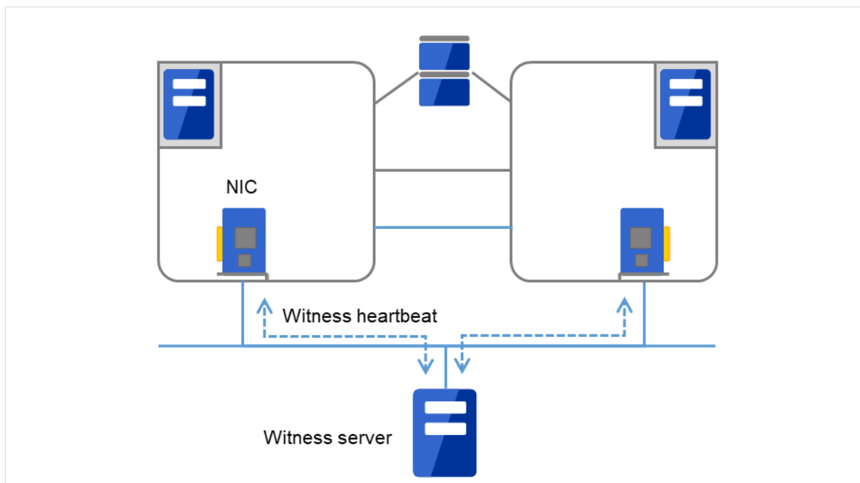
Fig. 3.7: Witness heartbeat
